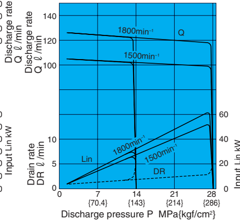
Pressure - Flow Rate Characteristics
